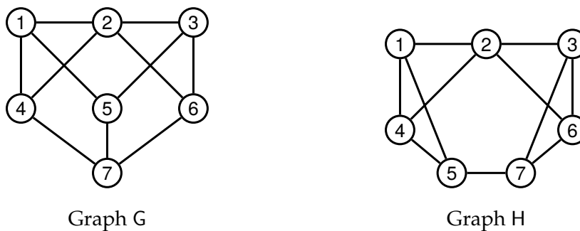
FIGURE 3.3: Graphs G and H give a counterexample to the converse of theorem 3.5 , since they have the same walk matrix but different CDC's.
