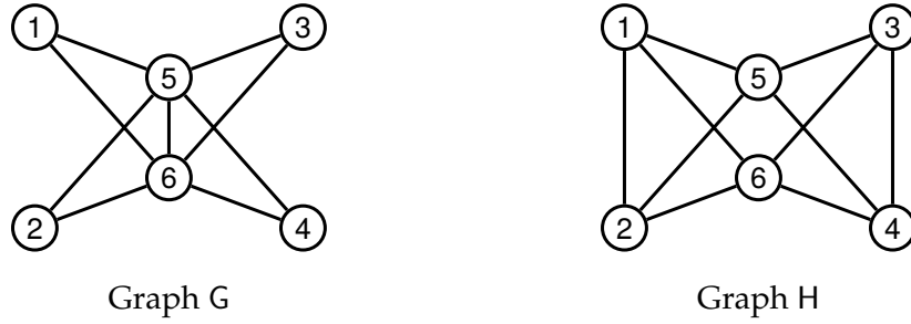
FIGURE 3.6: Graphs G and H have related walk matrices.
